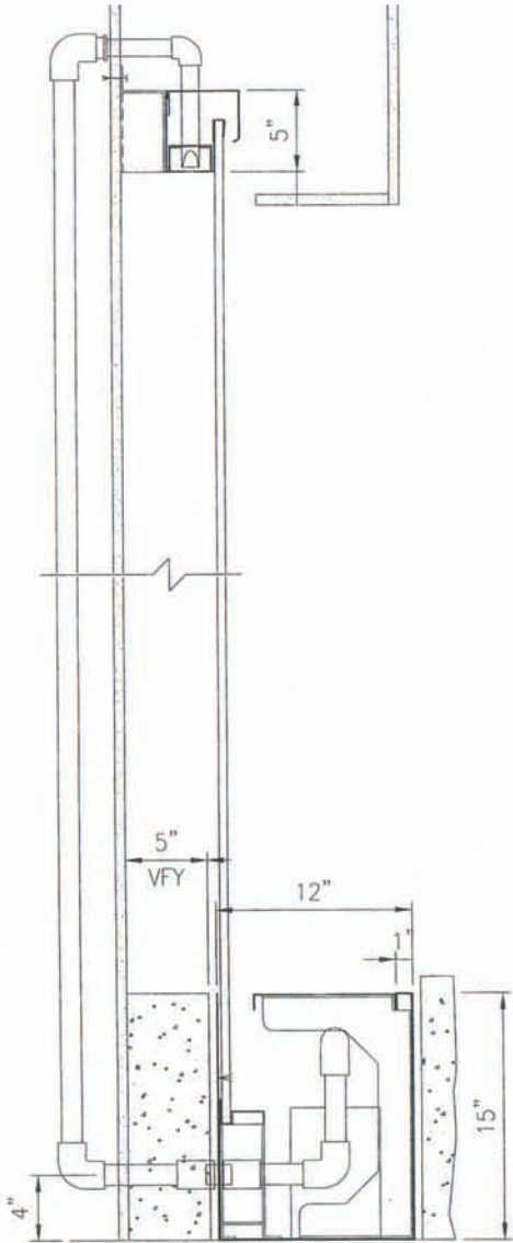
Example of plumbing through the wall for "floating" features
