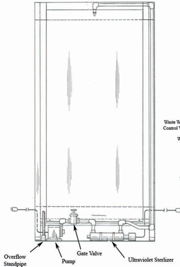
Example of internal plumbing for free standing and wall features
