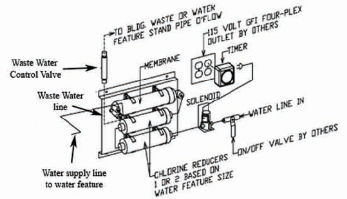
Reverse Osmosis System Setup
